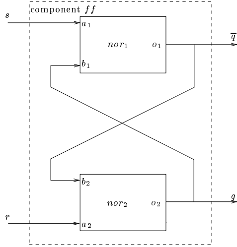
Figure 7.2: RS-flip-flop example
