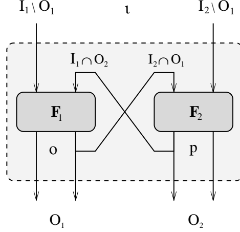
Figure 5.2: Binary composition
