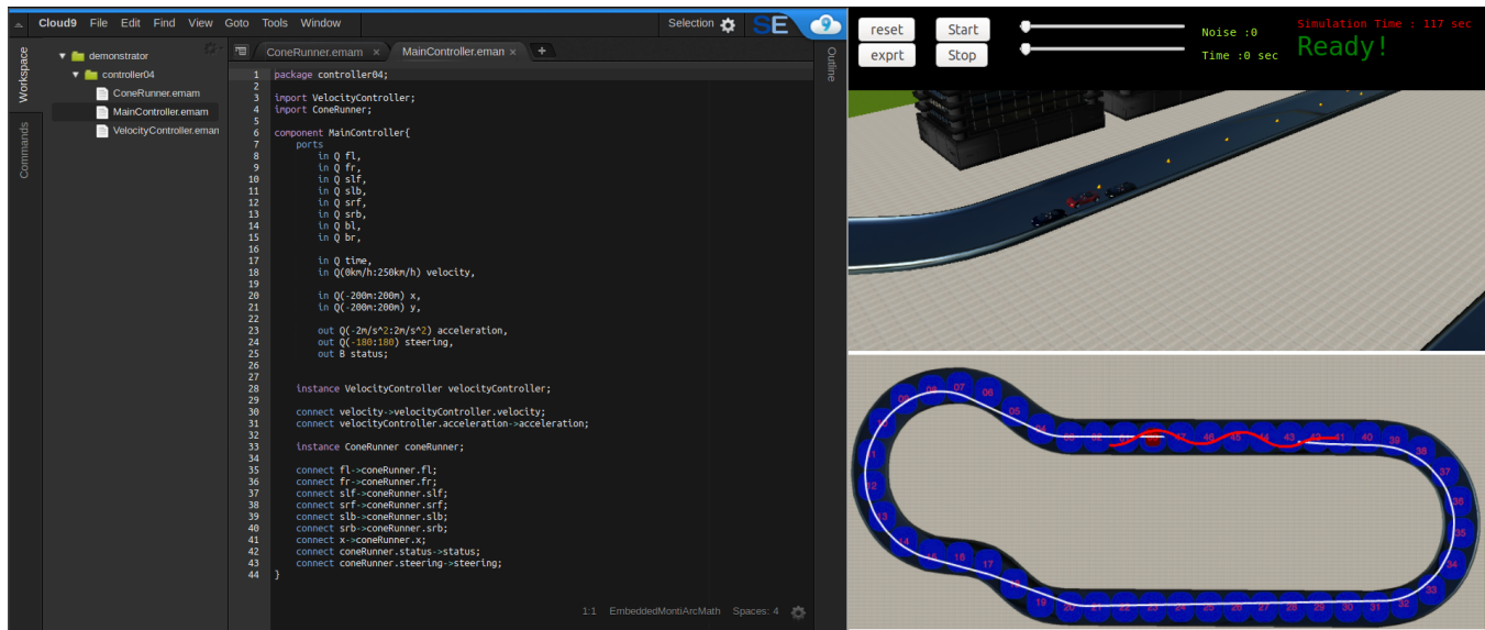
Figure 3: Screenshot of Tutorial Environment: left IDE, right top: 3D visualization, right bottom: trajectory
