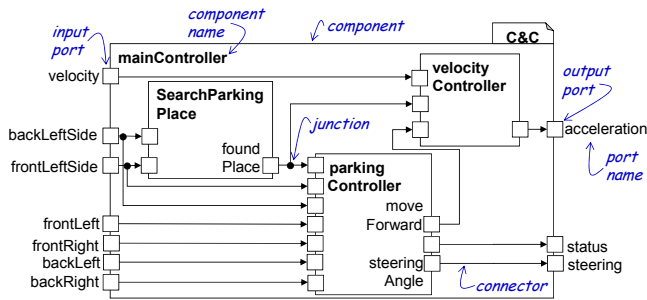
Figure 4: Graphical C&amp;C model of Listing 1 and Listing 2
