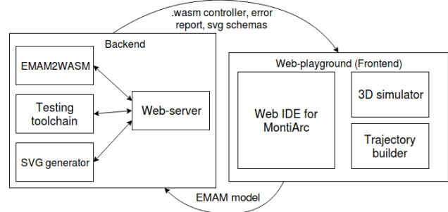
Figure 2: Architecture of C&C online tutorial platform.
