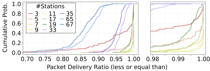
Fig. 4. Empirical distr. function of packet delivery ratios for different number of stations. Each number of stations simulated for 100 seeds. The right plot enlarges the region between 0.98 and 1.00 for better visibility.
