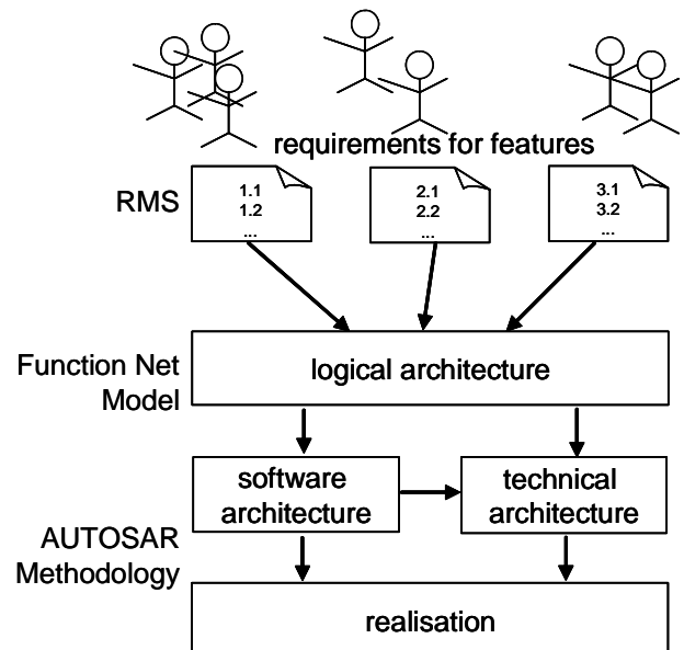
Figure 1 Development Process
