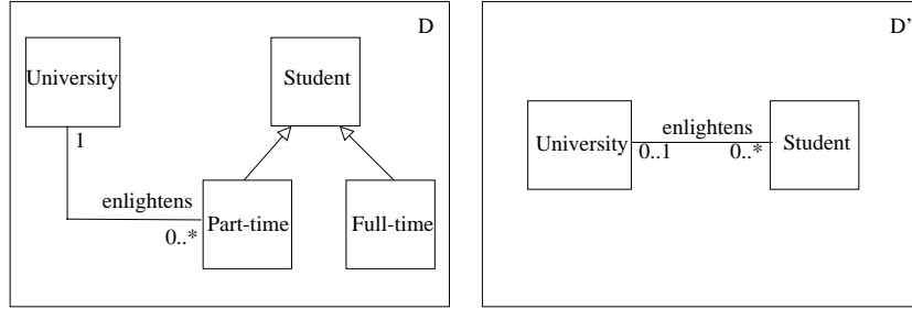
Fig. 1. Transforming a Class Diagram D to D' to derive information
