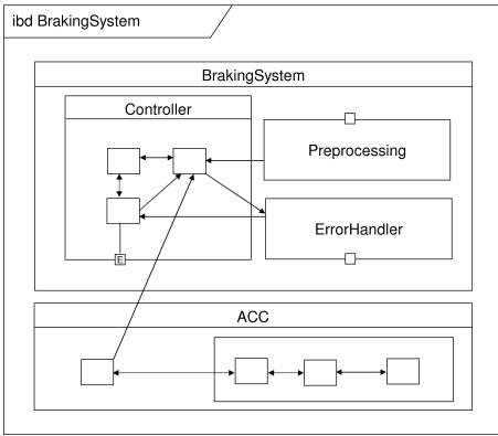
Figure 3. Excerpt from an automotive function net (Signals are omitted to enhance the readability)
