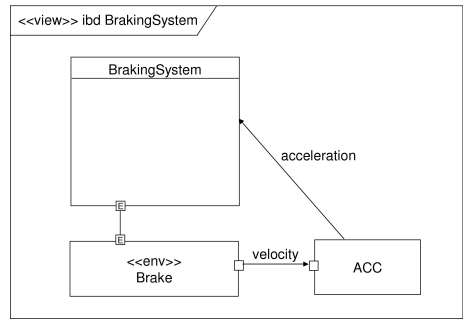
Figure 4. View of the automotive function net describing the braking system and its environment
