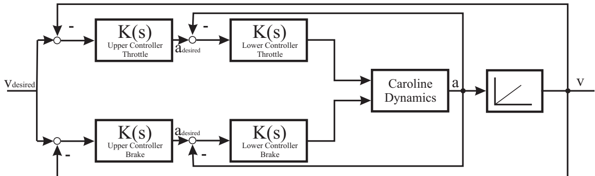
Figure 33: Block diagram of the longitudinal controller.
