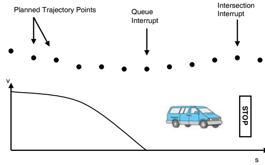
Figure 31: Interrupt example.
