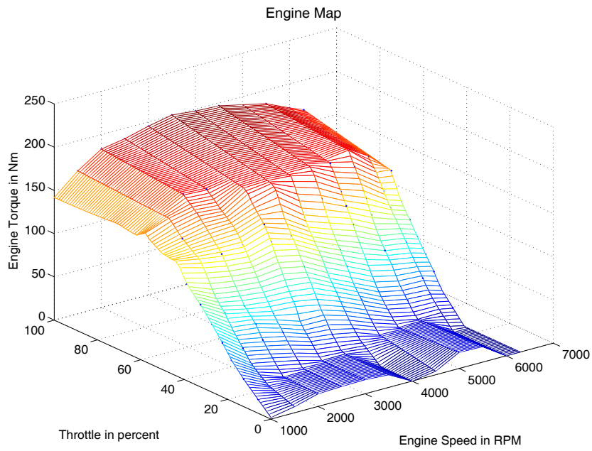
Figure 34: Engine map.
