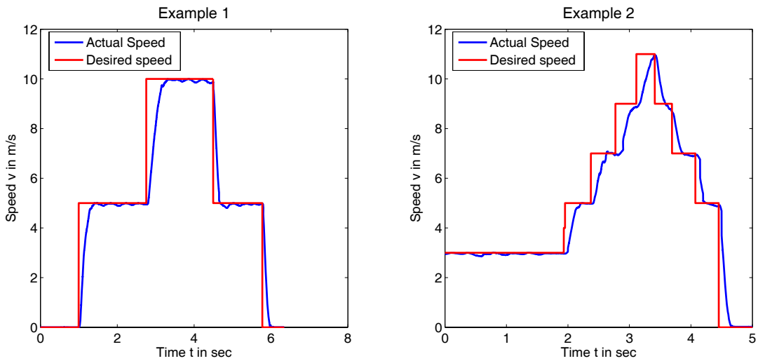
Figure 35: Performance of the longitudinal controller.
