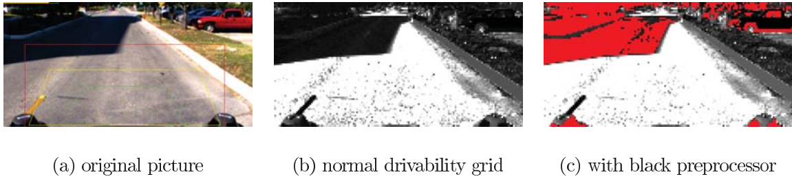
Figure 25: The results with black preprocessor. The picture in the center (b) shows the classification results without the black processor. In picture on the far right (c) the critical region is classified as unknown (red).
