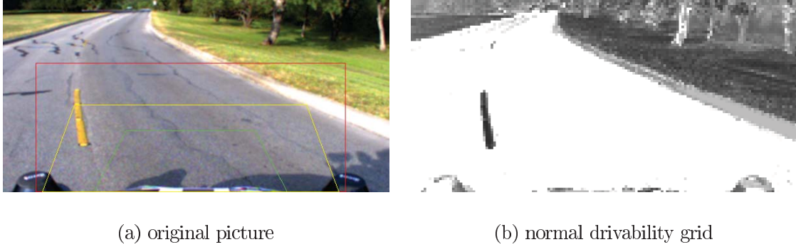
Figure 20: The drivability grid (b) depicts the output of algorithm, the results differ from black (undrivable) to white (drivable) . A yellow line (a) is marked as undrivable (b, black) because the color differs by too much from the street color.
